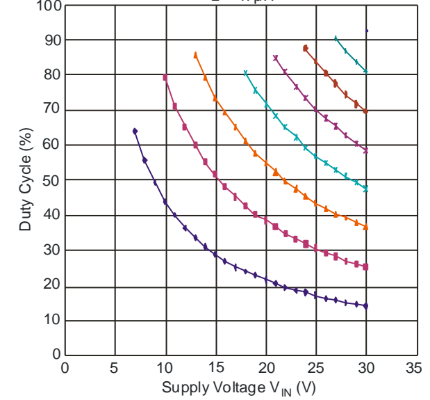
ZXLD1360 Duty Cycle L = 47 \mu H
