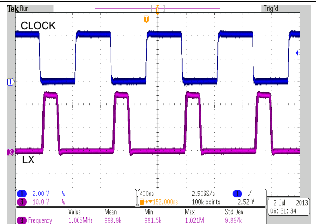
Figure 47. Clock Synchronization at 1 MHz
