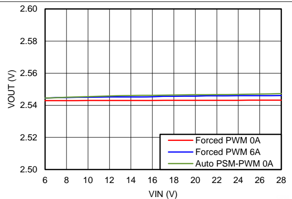
Figure 7. Buck Line Regulation, V_{OUT} = 2.5\text{ V}
