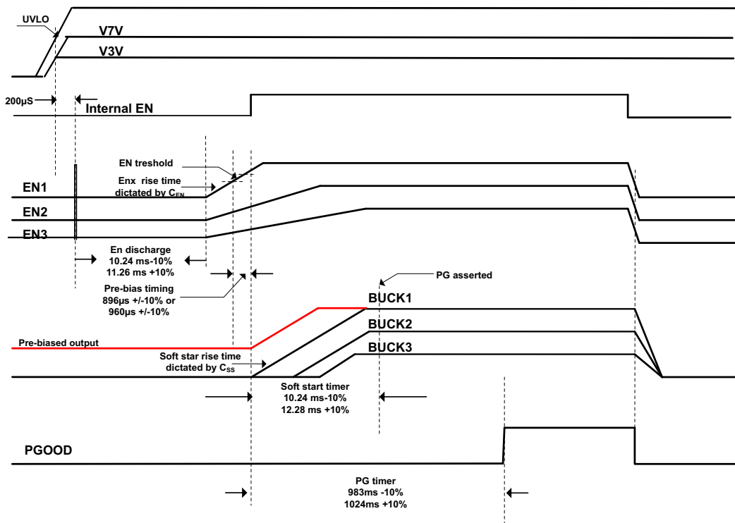
Figure 20. TPS65251-x Timing Diagram
