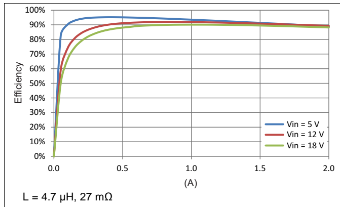
Figure 13. Efficiency, Forced PWM
