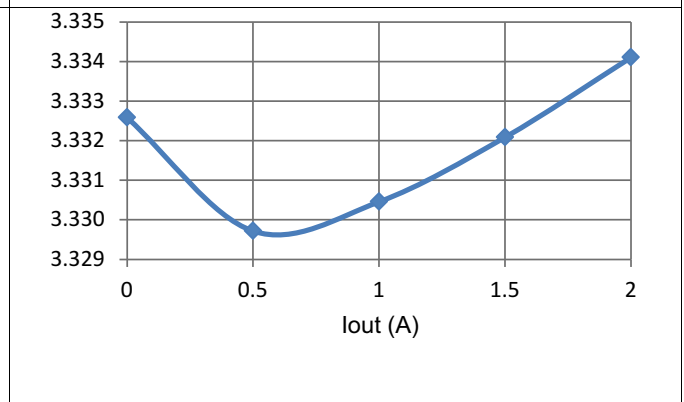
Figure 16. Load Regulation, 25^\circ\text{C} , 1% 100-PPM Resistor
