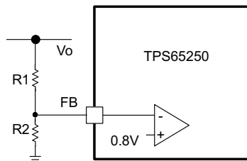
Figure 31. Voltage Divider Circuit
