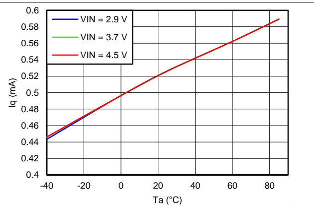
Figure 3. Quiescent Current
