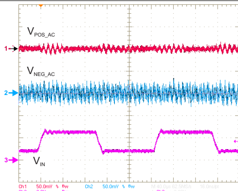
Figure 96. Line Transient — I OUT = 100 mA SYNC = HIGH — ΔV IN = 1.7 V
