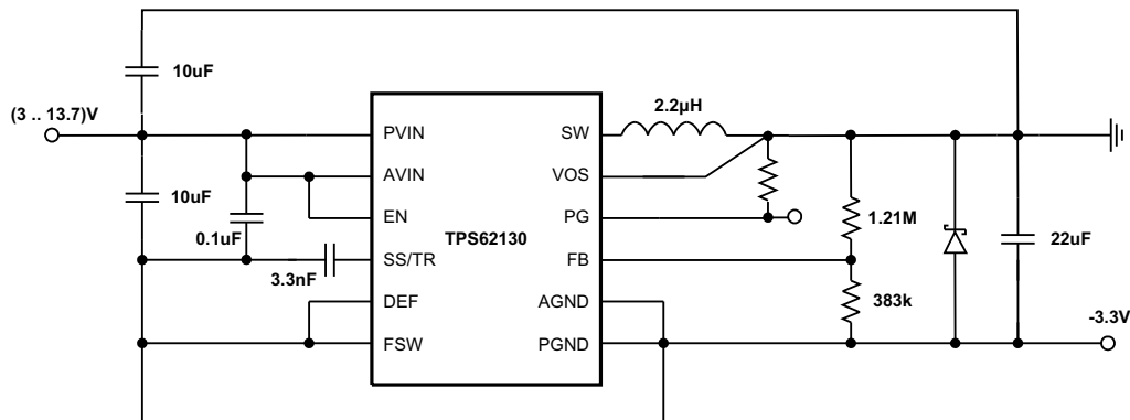
Figure 48. –3.3 V Inverting Power Supply
