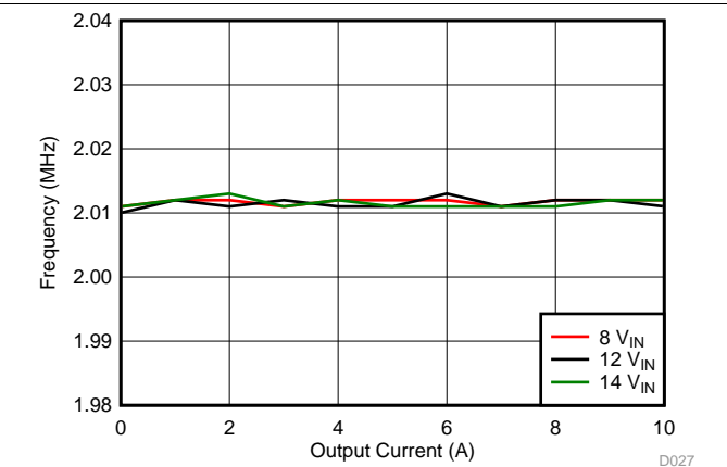
Figure 26. Frequency vs Output Current
