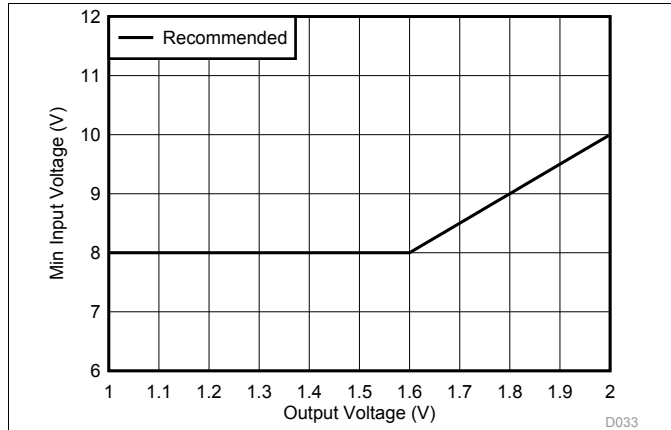
Figure 25. Min Input Voltage vs Output Voltage
