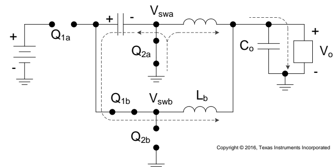
Figure 45. Phase B High Side MOSFET On
