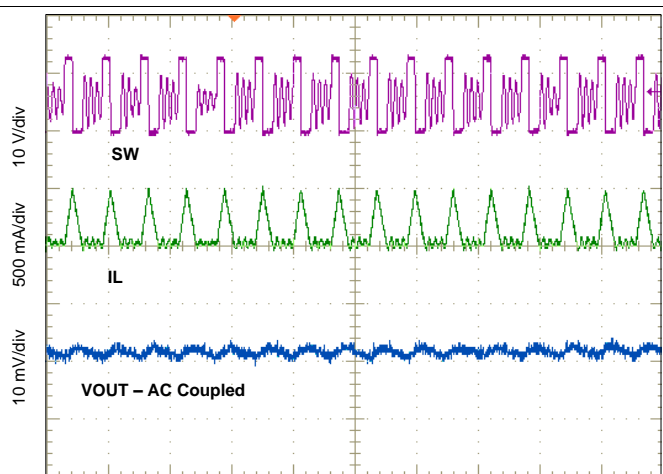
Time = 4 \mu s/div Figure 56. Output Ripple DCM
