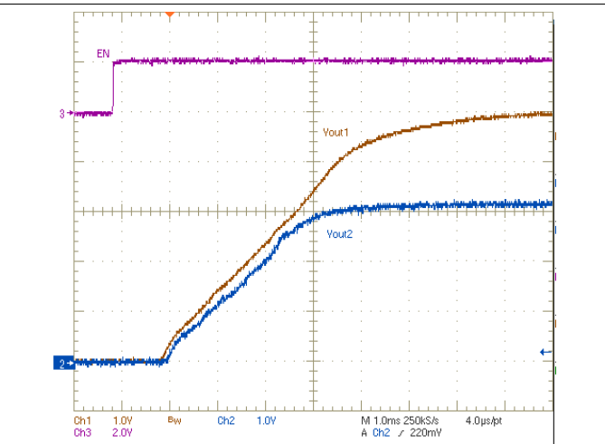
Figure 35. Ratio-Metric Startup with Tracking Resistors
