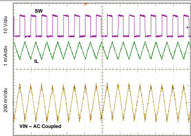
Time = 4 \mu s/div Figure 58. Input Ripple CCM
