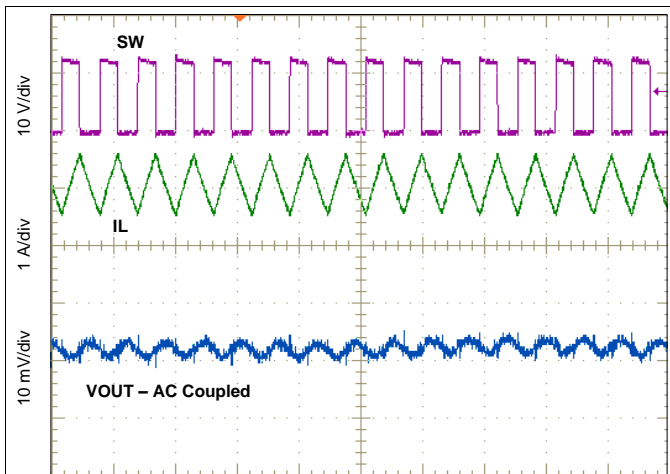
Time = 4 \mu s/div Figure 55. Output Ripple CCM
