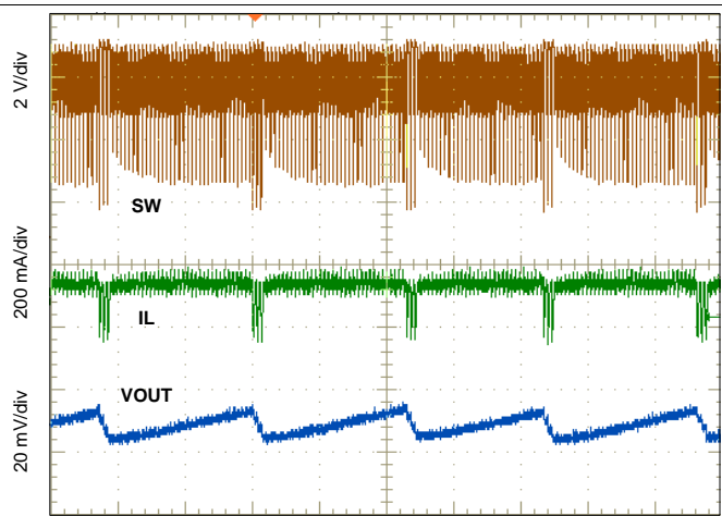
Time = 40 \mu s/div Figure 60. Low Dropout Operation
