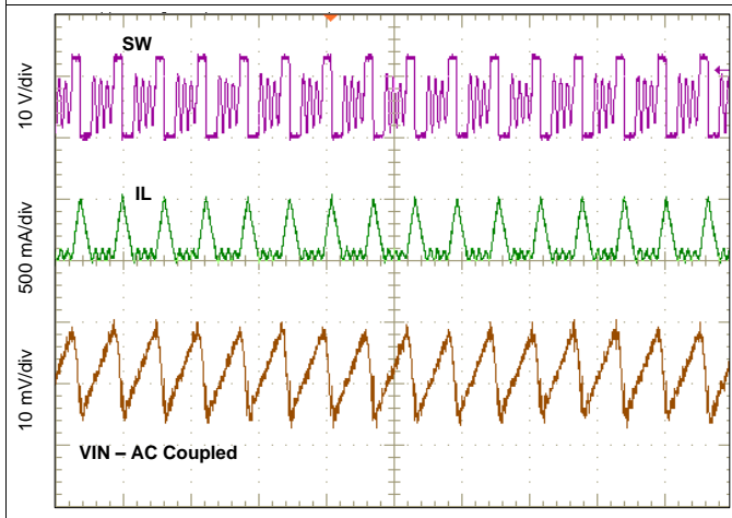
Time = 4 \mu s/div Figure 59. Input Ripple DCM
