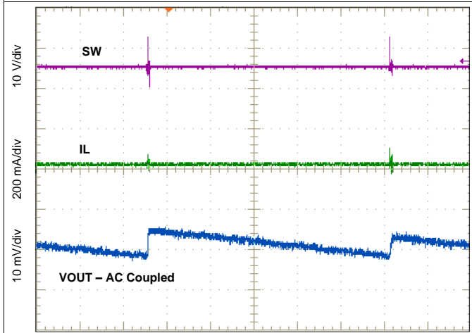
Time = 1 ms/div Figure 57. Output Ripple PSM
