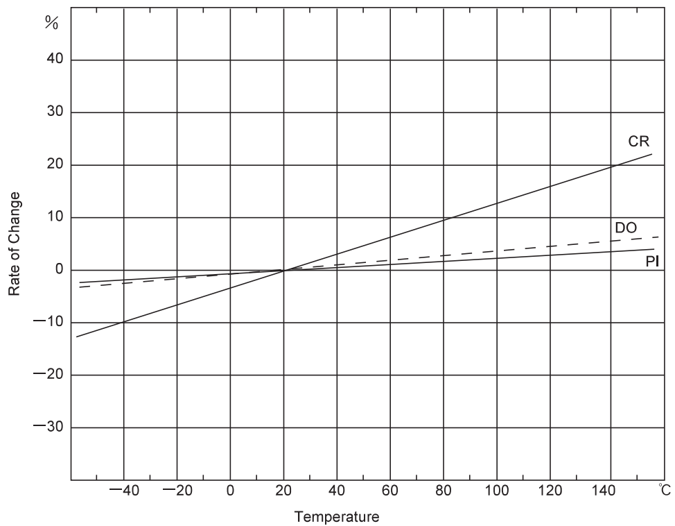
(1) Temperature Characteristics
