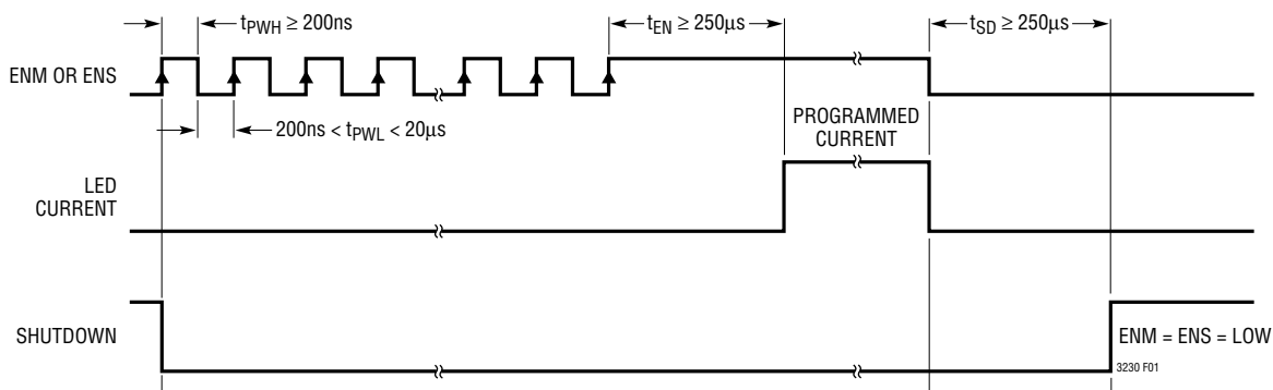
Figure 1. Current Programming Timing Diagram
