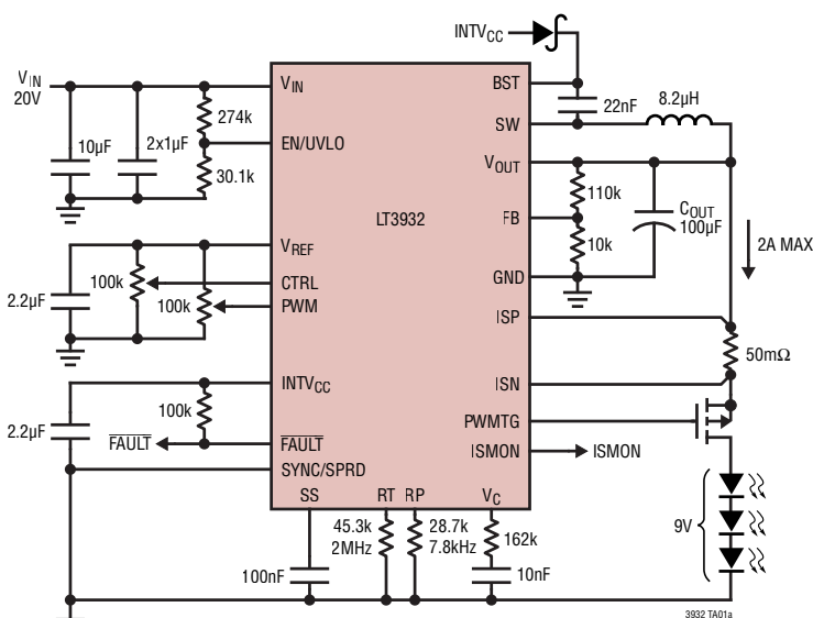
2A LED Driver with Internal PWM Dimming
