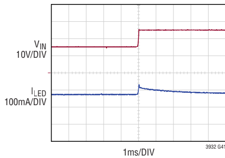
Input Voltage Transient Response
