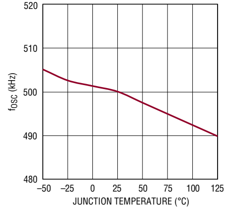
Oscillator Frequency f_{OSC} vs Temperature
