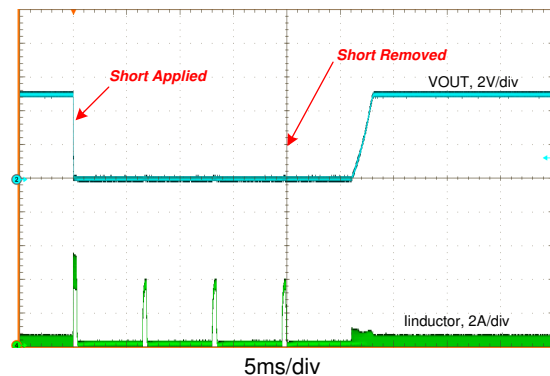
Figure 14. Short-Circuit Transient and Recovery
