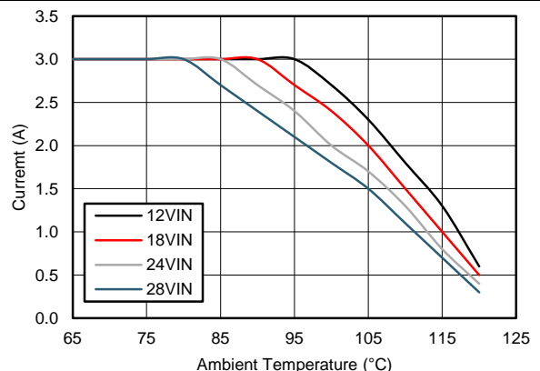
V_{OUT} = 5\text{ V} F_S = 1\text{ MHz} \theta_{JA} = 20^{\circ}\text{C/W}
