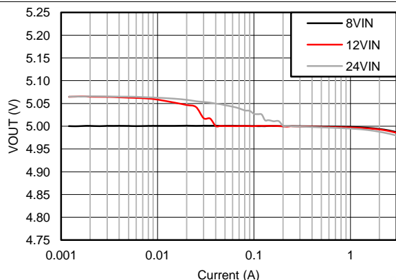
V_{OUT} = 5\text{ V} F_S = 1\text{ MHz}
