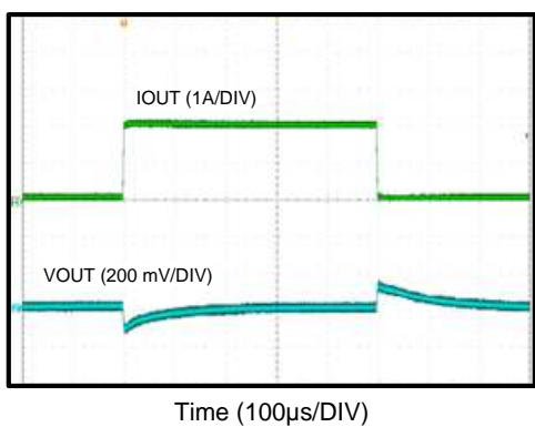
V_{OUT} = 5\text{ V} F_S = 1\text{ MHz}
