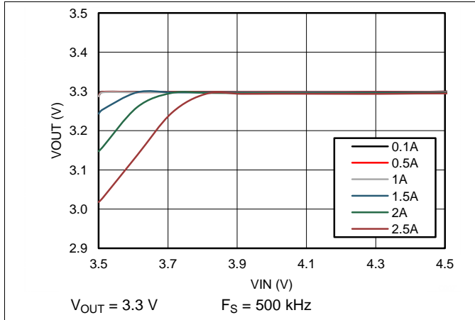
Figure 61. Dropout Curve
