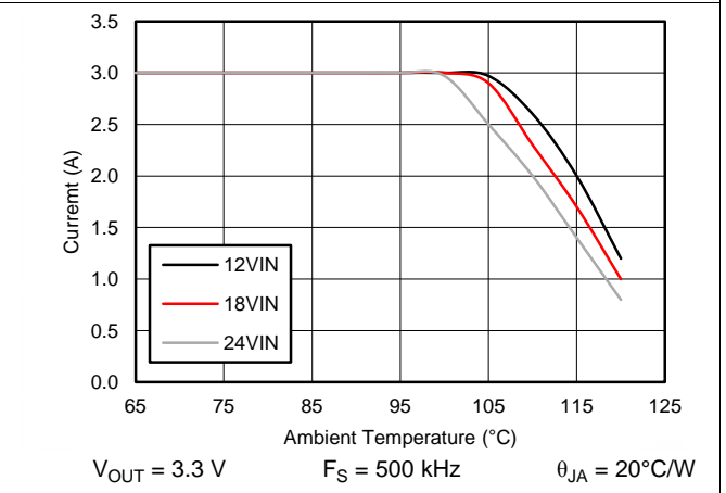
Figure 66. Derating Curve
