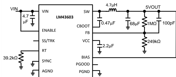
V_{OUT} = 5\text{ V} F_S = 1\text{ MHz}
