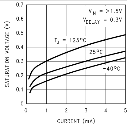
Figure 11. Flag Saturation Voltage
