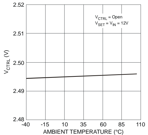
Figure 6 V_{CTRL} vs. Temperature
