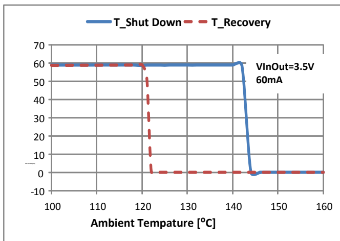
Figure 24 THSD of 60mA Current Option
