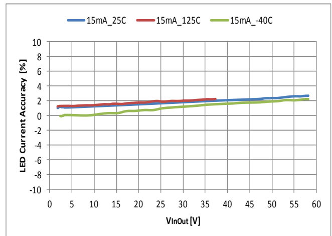
Figure 17 LED Current Accuracy (%) vs. VinOut across Temperature
