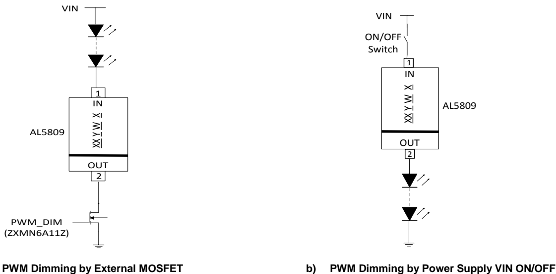
Figure 4 PWM Dimming
