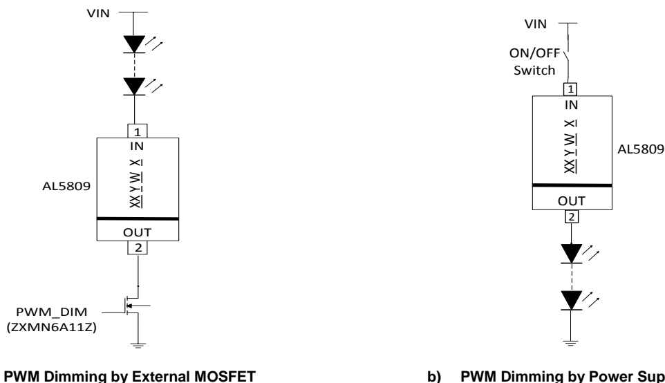
Figure 4 PWM Dimming
