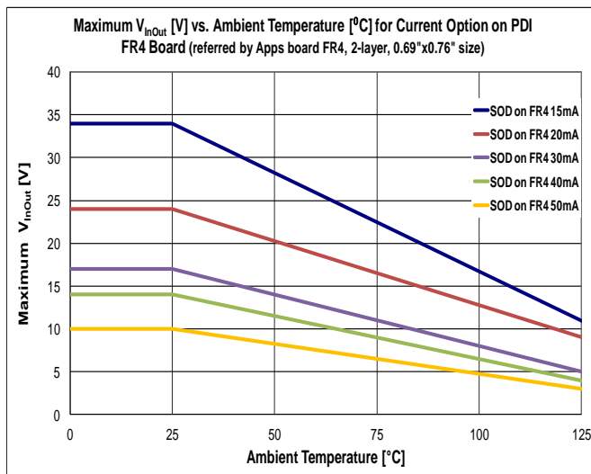
Figure 11 Maximum V INOut vs. Temperature
